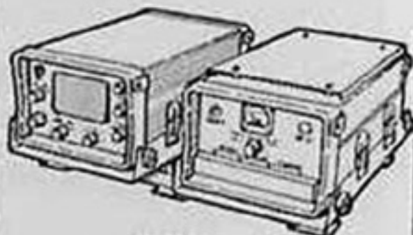
RT422B Fixed/mobile SSB Radiotelephone Solid State plus 3 tubes 125W PEP 4 Channels 2-16 MHz
