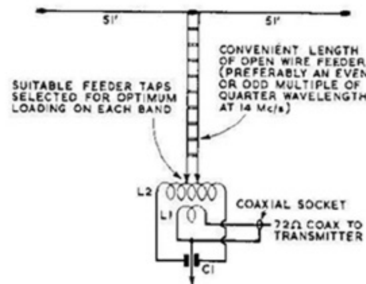
Fig. 2. Multiband aerial with tuned feeders.
